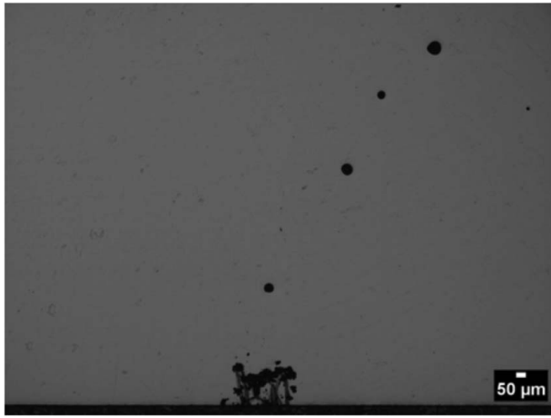
Fig. 4 Interface of shell and core regions within Sample 6. Note the mark at the bottom center of the image was added to indicate the location of the interface region and is not part of the microstructure.
