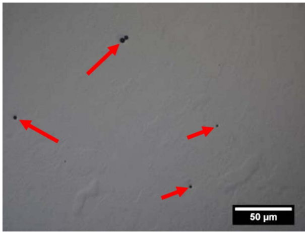
Fig. 2 Representative image showing porosity within samples printed with the OEM recommended setting of 200 W laser power
