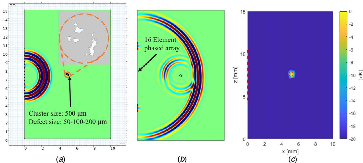
Fig. 8 (a and b) Two time snapshots showing the propagation and reflection of longitudinal waves generated by a single phased array element and reflected from a cluster of defects of size 500\ \mu\text{m} located at 5 mm depth. (c) The TFM image as constructed from the FMC data of the phased array shown in (b). The cluster of defects location is highlighted with a circle.
