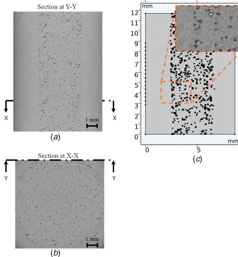
Fig. 5 (a) Front and (b) top cross sections of an X-ray CT scan of Sample 2 showing a uniform distribution of the defects in the core region. (c) Defect geometry as generated from the XCT images to be used in FEM wave propagation simulations.
