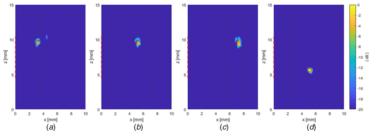
Fig. 9 TFM images generated for clusters of defects located at +2 mm from the center of the array and a depth of (a) 3 mm, (b) 5 mm, and (c) 7 mm. A cluster at -2 mm and a depth of 5 mm is shown in (d). In all cases, the defect cluster location is highlighted with a circle, and the phased array location is highlighted with a dashed line.
