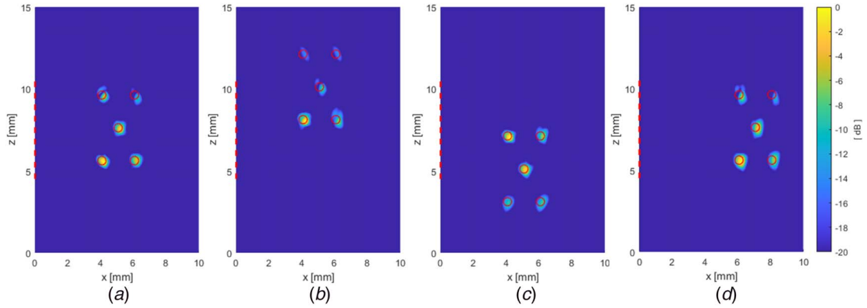
Fig. 10 TFM images generated for multiple clusters of defects present in the same sample. The locations of the defect clusters are highlighted with circles, and the phased array location is highlighted with a dashed line. The probe is centered about the defects in (a), shifted by -2.5 mm in the z -direction in (b) and by +2.5 mm in (c). The depth of the defects is shifted by 2.5 mm in the x -direction in (d).
