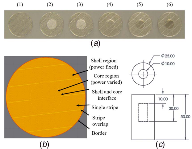
Fig. 1 (a) Top view of the SLM samples taken during their 3D printing. The laser power used at the core region is summarized in Table 1. Note that Sample 1 was printed without the shell and core regions distinction. (b) Different regions as defined during the 3D printing of the SLM samples. (c) Schematic showing the geometry of the samples and the dimensions of the internal defect region (dimensions are in millimeters).
