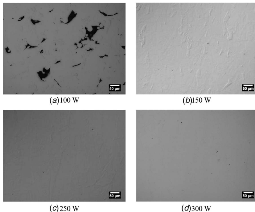
Fig. 3 Core region optical images of Samples: (a) 2–100 W, (b) 3–150 W, (c) 5–250 W, and (d) 6–300 W
