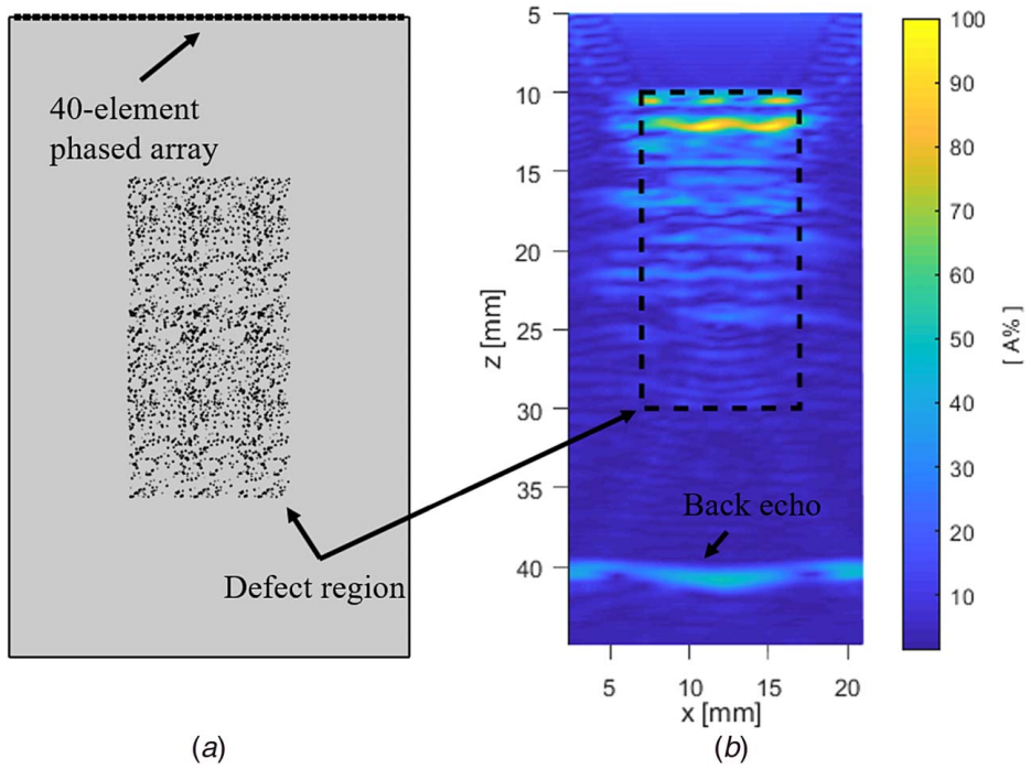
Fig. 7 (a) Constructed geometry for visualizing the wave propagation through Sample 2. The defect geometry was extracted from XCT images. (b) Linear B-scan image of the sample generated by a 40-element array with an aperture of eight elements.
